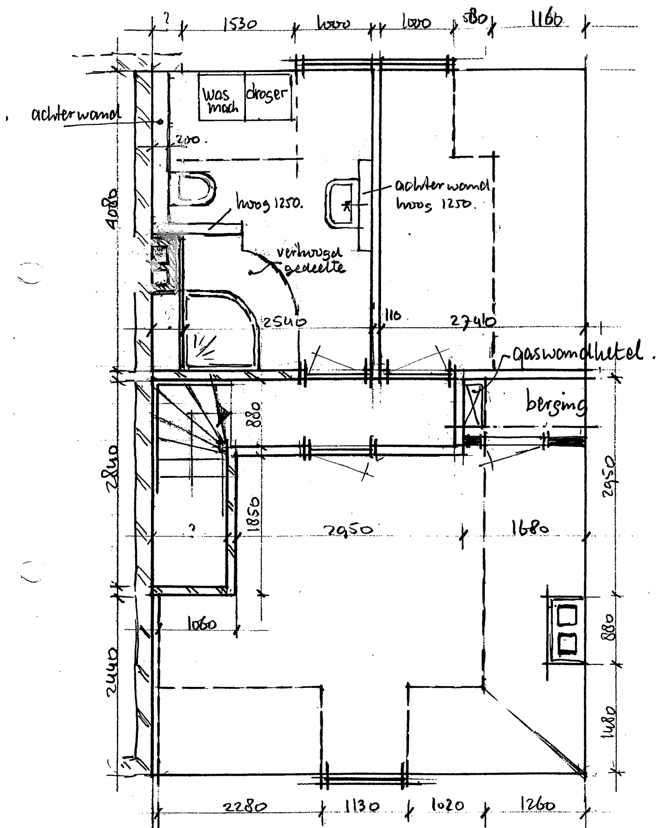
ZOLDERVERDIEPING. schaal 1:50.
